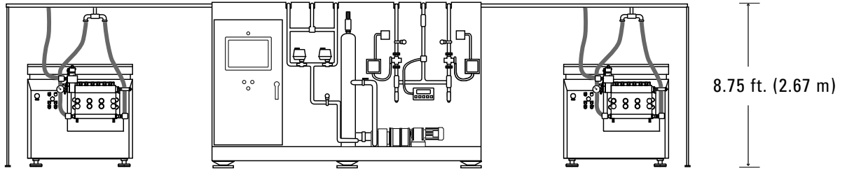
SIDE ELEVATION
